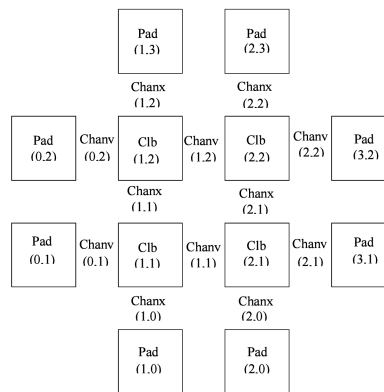
Fig. 3.1: FPGA co-ordinate system.
